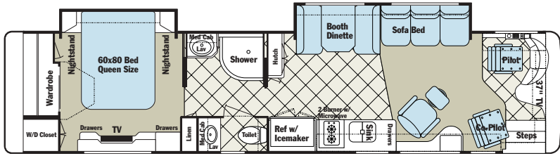
U320/3820 PBBD Private Bath, Bed Slide (Driver Side)
