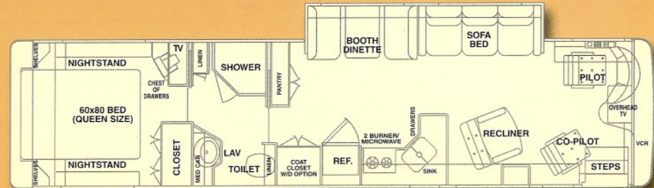
3610 U270 WTFS (Walk Through Bath, Front Slide)
