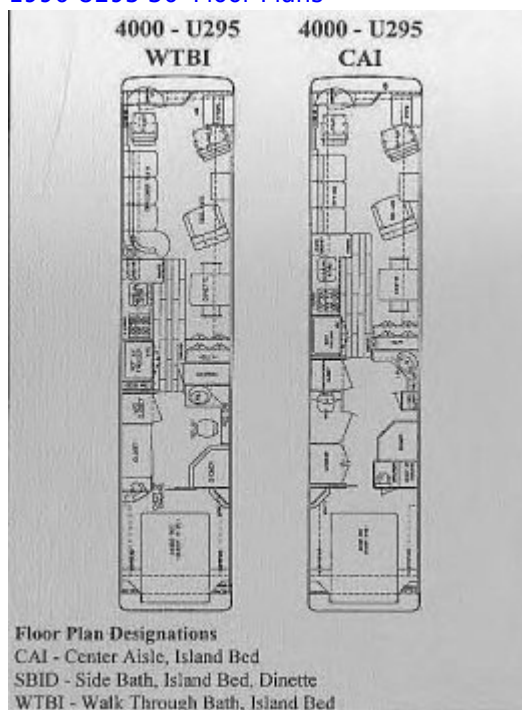
1996 U295 40' Floor Plans
