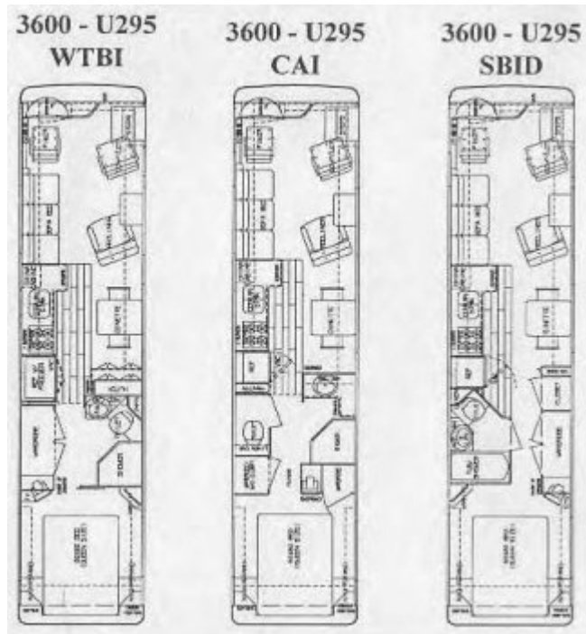
1996 U295 36' Floor Plans
